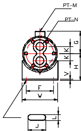
MOUNTING HOLE
